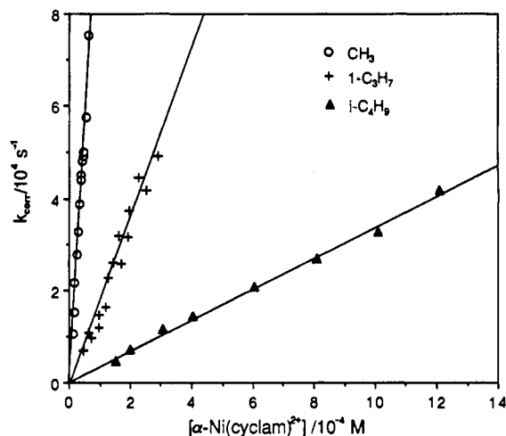
Figure 1. Plots of kinetic data for the colligation reactions between alkyl radicals and \alpha - Ni(\text{cyclam})^{2+} . The data are shown as a plot of k_{corr} vs [\alpha\text{-Ni}(\text{cyclam})^{2+}] in accordance with eq 9.
