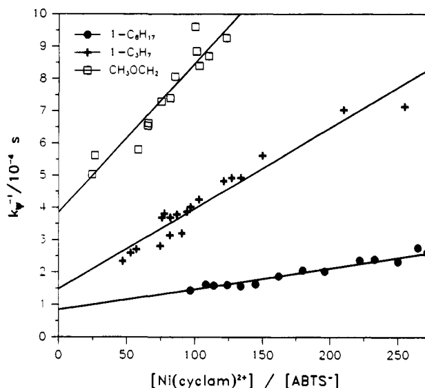
Figure 2. Plots of 1/k_{\psi} vs [\text{Ni(cyclam)}^{2+}]/[\text{ABTS}^-] for the reactions of \beta\text{-Ni(cyclam)}^{2+} . A linear relation is found, as in eq 11.
